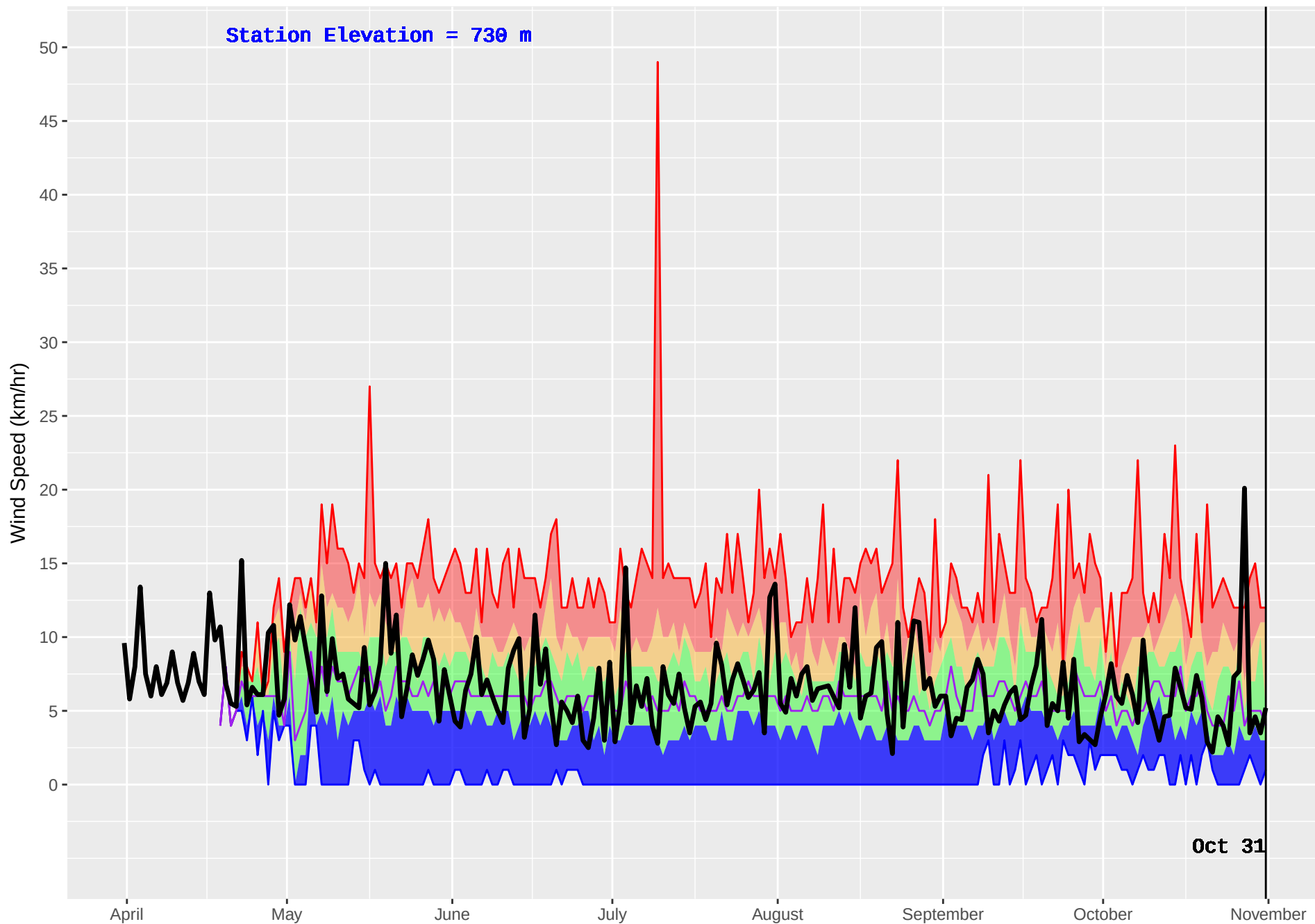
BOYA LAKE (445) : Historical (1985–2016) and Current (2017) Noon Wind Speed
