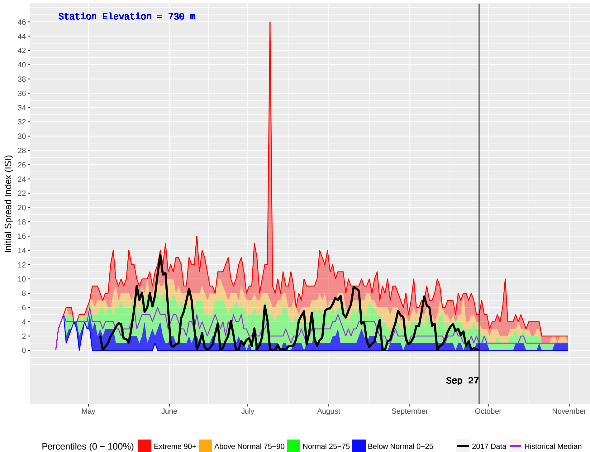
BOYA LAKE (445) : Historical (1985–2016) and Current (2017) Noon Initial Spread Index (ISI)
