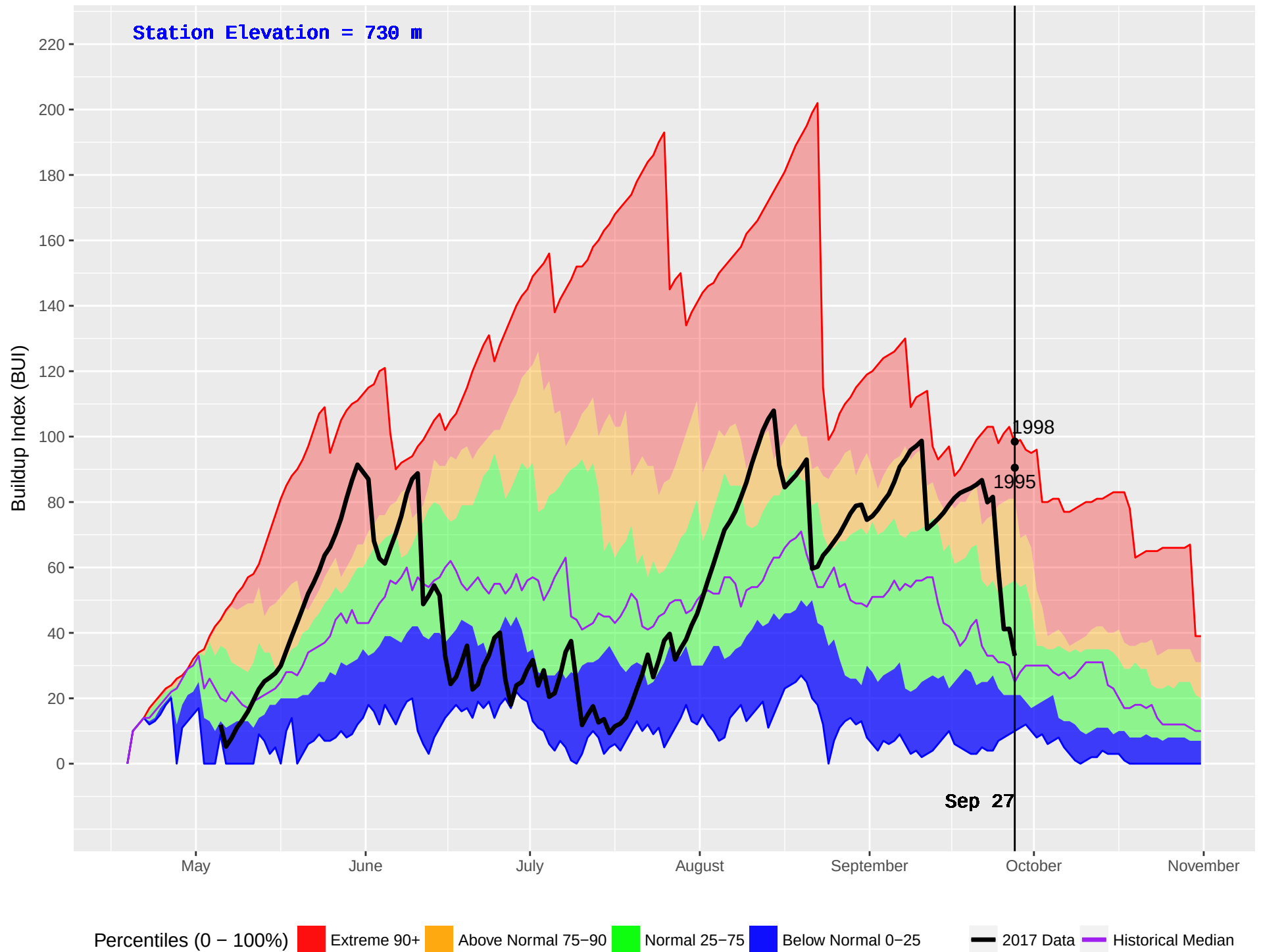
BOYA LAKE (445) : Historical (1985–2016) and Current (2017) Noon Buildup Index (BUI)
