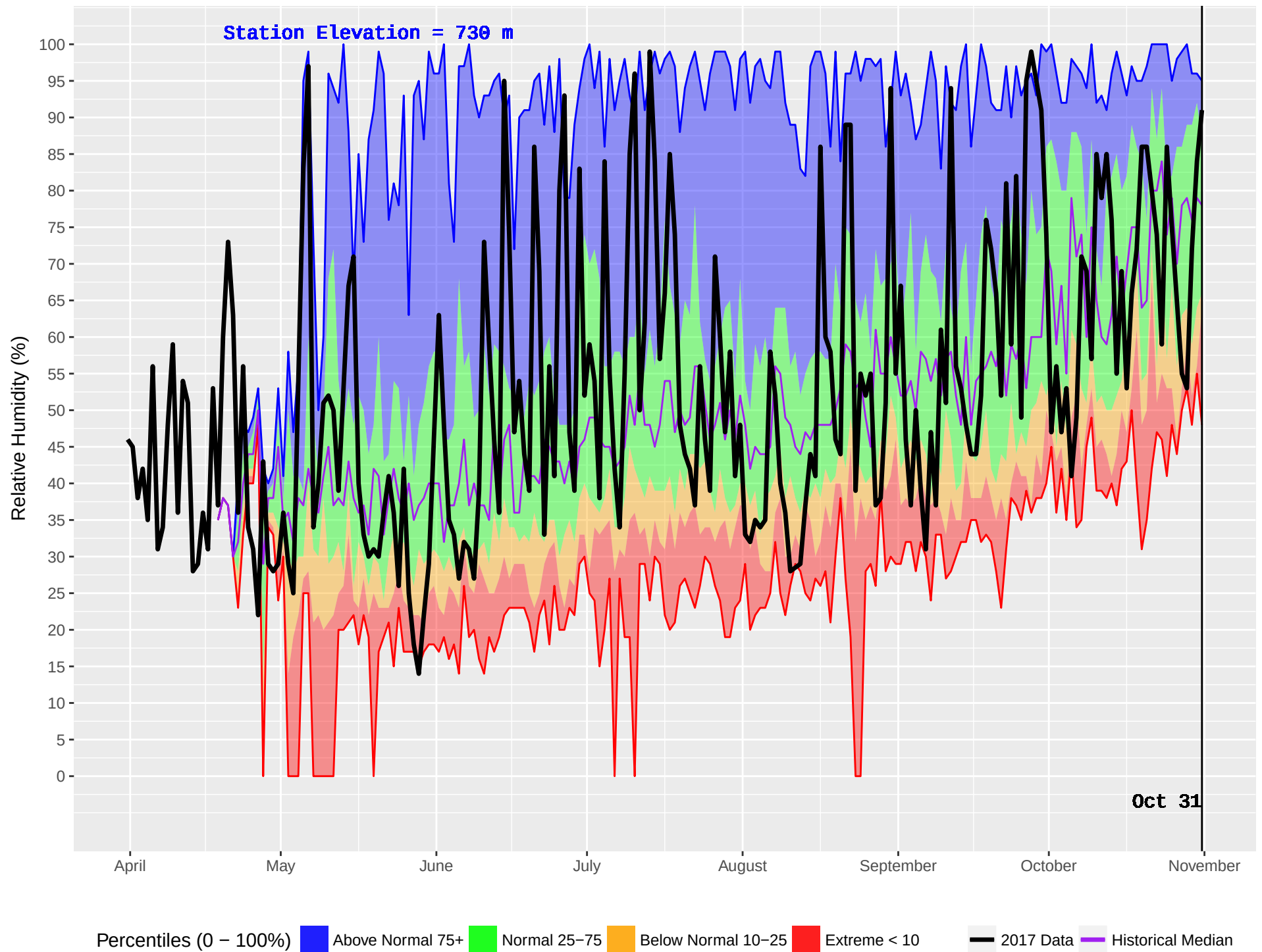
BOYA LAKE (445) : Historical (1985–2016) and Current (2017) Noon Relative Humidity
