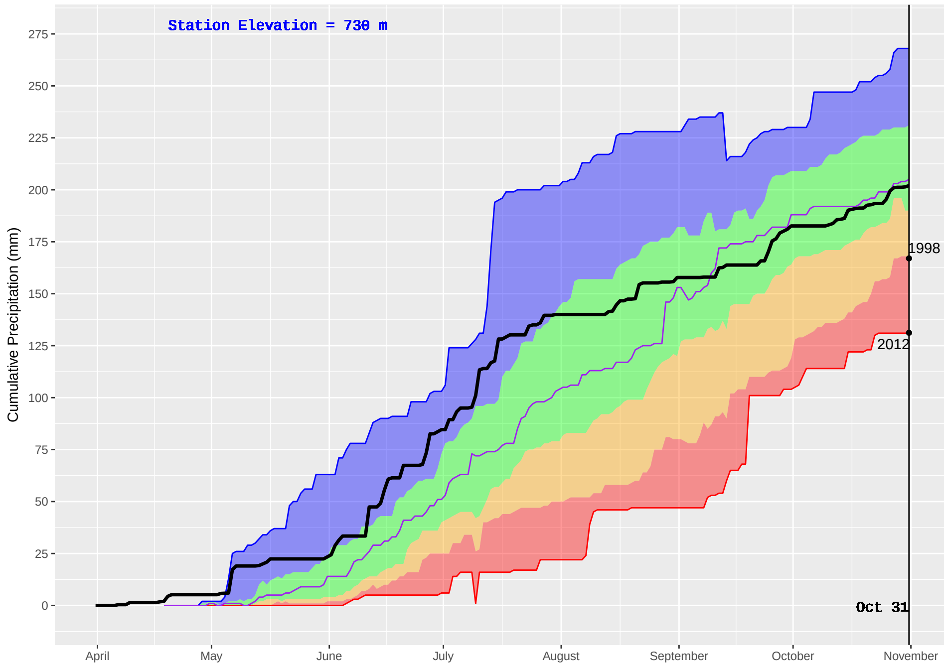
BOYA LAKE (445) : Historical (1985–2016) and Current (2017) Noon Cumulative Precipitation
